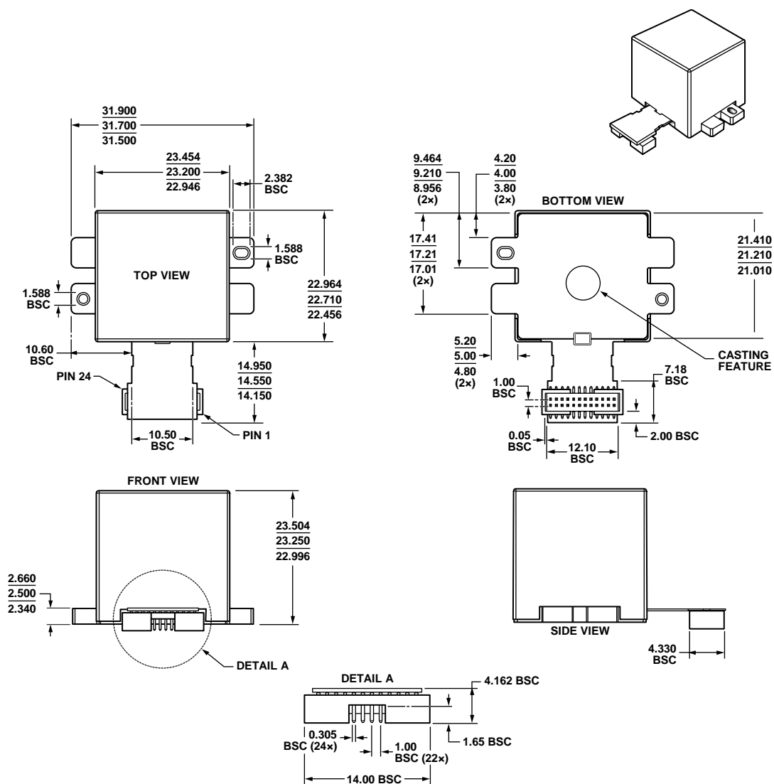
Figure 19. 24-Lead Module with Connector Interface (ML-24-2)
