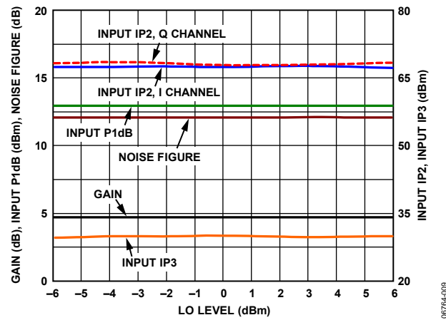
Figure 13. Conversion Gain, Noise Figure, IIP3, IIP2, and IP1dB vs. LO Level, f_{RF} = 140 MHz
