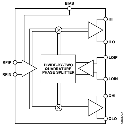
Figure 49. Block Diagram
