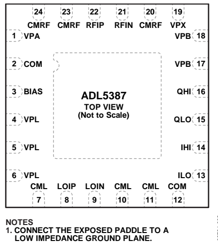
Figure 2. Pin Configuration
