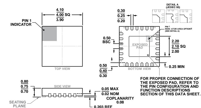
COMPLIANT TO JEDEC STANDARDS MO-220-WGGD-8. Figure 47. 24-Lead Lead Frame Chip Scale Package [LFCSP] 4 mm × 4 mm Body and 0.75 mm Package Height (CP-24-10) Dimensions shown in millimeters
