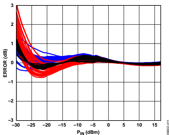
Figure 12. V_{ENV} Output Temperature Drift from +25°C, Three-Point Calibration for Multiple Devices at -40°C, +25°C, and +85°C at 900 MHz
