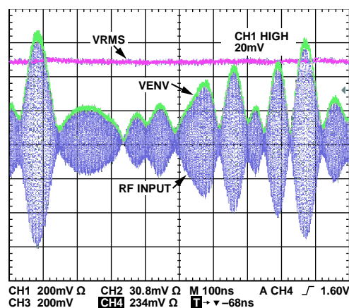
Figure 2. RMS and Envelope Response to a 20 MHz QPSK-Based LTE Carrier (Test Model E-TM1_1_20MHz)
