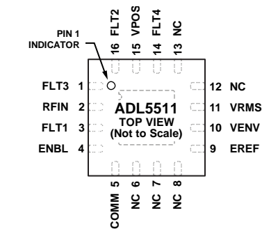
Figure 3. Pin Configuration
