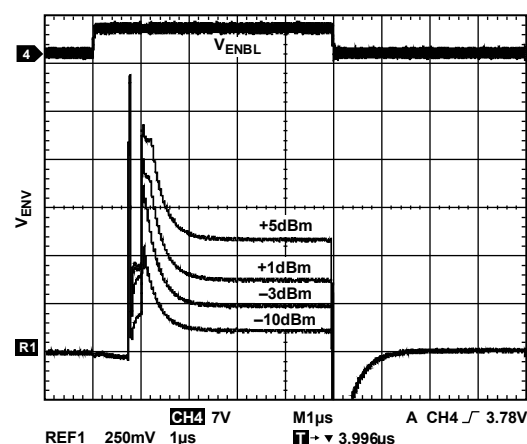
Figure 43. V_{ENV} Output Response to Enable Gating at Various RF Input Levels, 900 MHz Frequency
