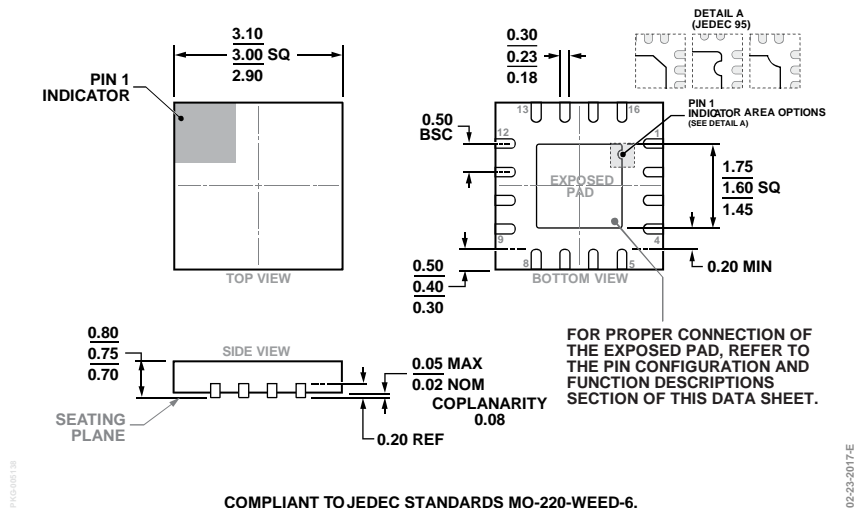
Figure 48. 16-Lead Lead Frame Chip Scale Package [LFCSP] 3 mm x 3 mm Body and 0.75 mm Package Height (CP-16-22) Dimensions shown in millimeters
