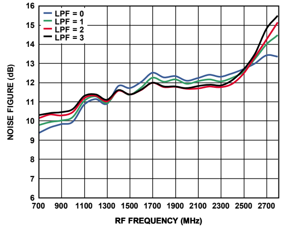
Figure 52. Noise Figure vs. RF Frequency for All LPF Settings, RFB and VGS Use Optimum Settings.
