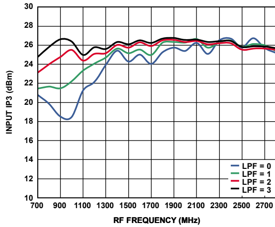
Figure 50. Input IP3 vs. RF Frequency for All LPF Settings, RFB and VGS Use Optimum Settings
