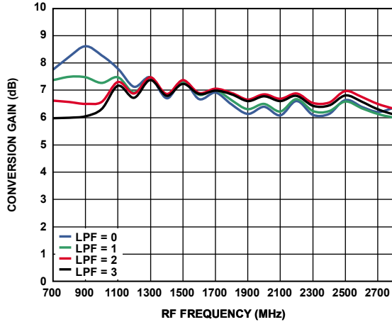
Figure 49. Conversion Gain vs. RF Frequency for All LPF Settings, RFB and VGS Use Optimum Settings
