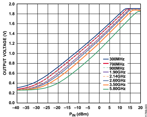
Figure 3. Typical V RMS vs. Input Level vs. Frequency (300 MHz to 5.8 GHz) at 25°C
