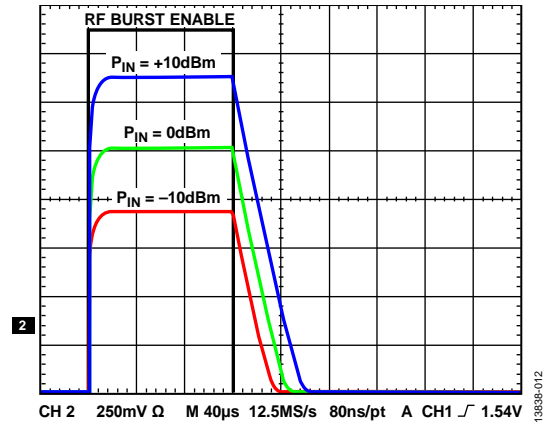
Figure 12. Output Response to RF Burst Input, Carrier Frequency = 900 MHz, C_{RMS} = 10\text{ nF} (see Figure 41 in the Test Circuits Section)
