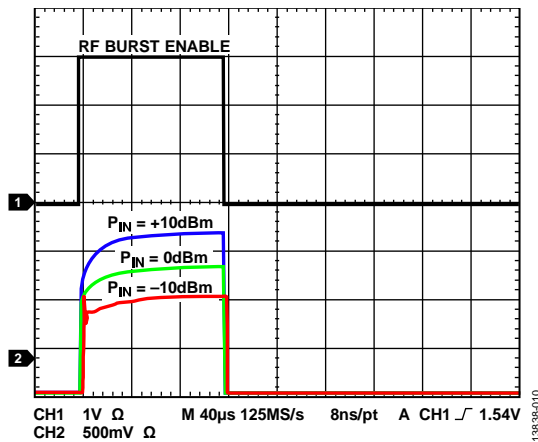
Figure 10. Output Response to Gating on ENBL Pin for Various RF Input Levels, Carrier Frequency = 900 MHz, C_{RMS} = 100\text{ nF}
