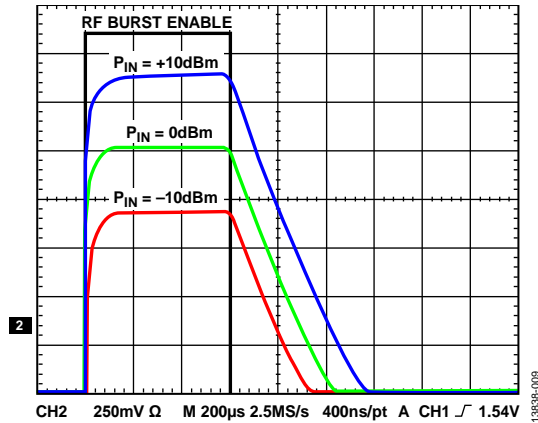
Figure 9. Output Response to RF Burst Input, Carrier Frequency = 900 MHz, C_{RMS} = 100\text{ nF} (see Figure 41 in the Test Circuits Section)
