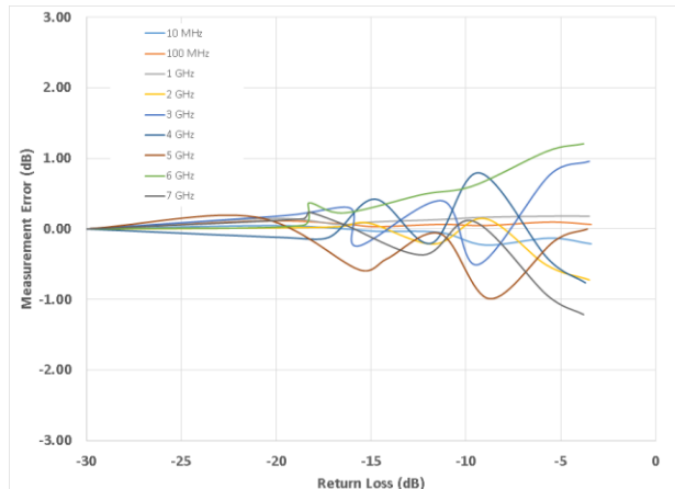
Figure 18. Power Measurement Error vs. Return Loss, Bridge Driven from RFIN with Varying Return Loss on RFOUT. VRMSF Output Voltage Calibrated with 50 ohm load on RFOUT
