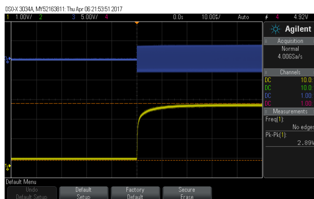
Figure 8. VRMSF Pulse Response to a 20 dBm RF Burst at 1 GHz Carrier Frequency. CRMS = 10 nF. Time base is 10 uS/div
