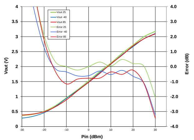
Figure 13. VRMSF vs. Input on RFIN at 3 GHz, 50 Ohm termination on RFOUT, 3-Point calibration at -10 dBm, +0 dBm and +25 dBm, TADJI=0V, TADJS=0.2 V
