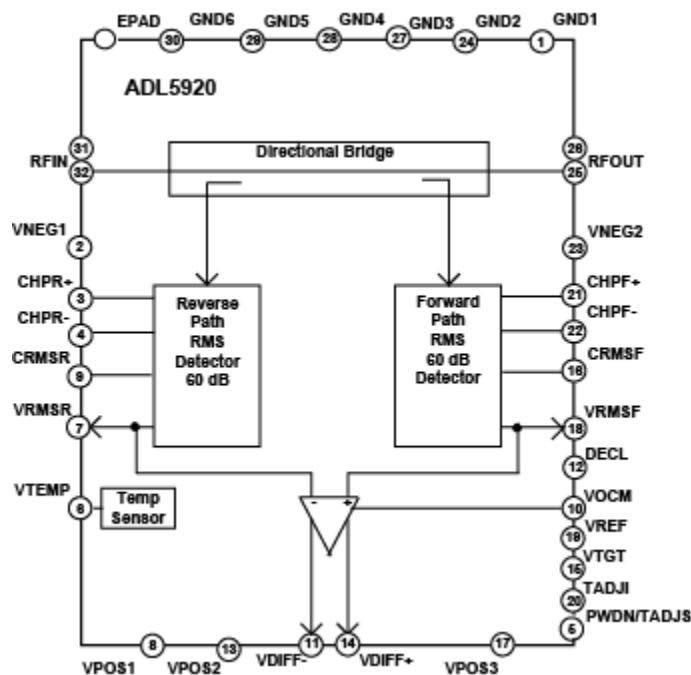
Figure 2. Pin Configuration
