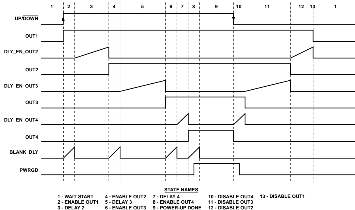
Figure 34. ADM1186-2 Typical Power-Up and Power-Down Sequence Waveforms with Corresponding State Names
