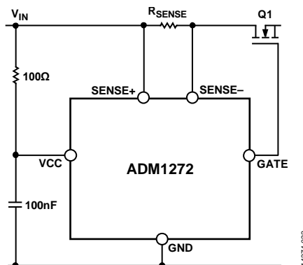
Figure 33. Reinforced Transient Glitch Protection Using an RC Network
