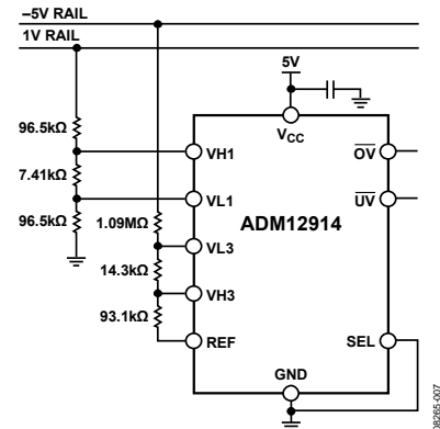
Figure 20. Positive and Negative Supply Monitor Example
