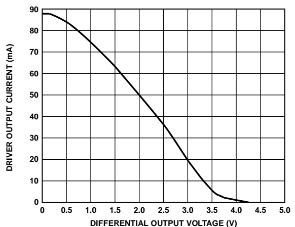
Figure 8. Driver Output Current vs. Differential Output Voltage
