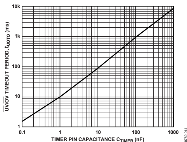
Figure 14. \overline{UV}/\overline{OV} Timeout Period vs. Capacitance
