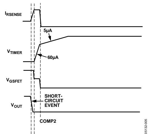
Figure 33. ADM4210-2 Latch Off After Overcurrent Fault
