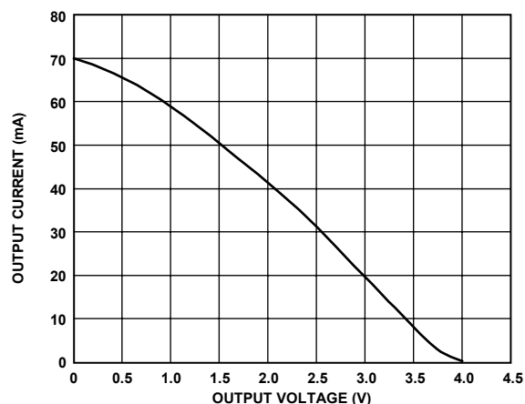
Figure 19. Output Current vs. Driver Differential Output Voltage
