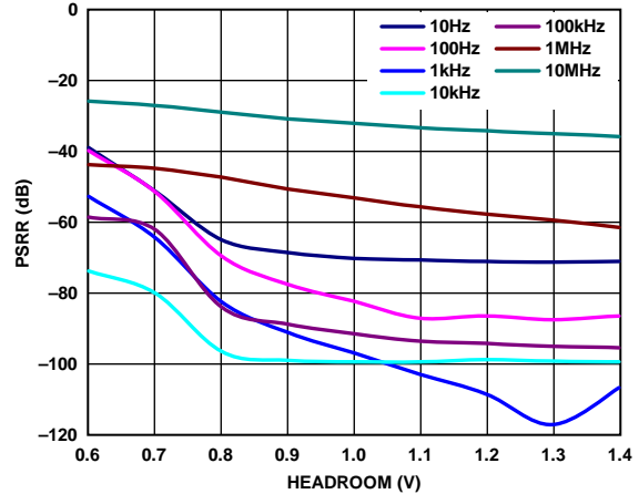
Figure 26. Power Supply Rejection Ratio (PSRR) vs. Headroom Voltage, ADM7151-02, V_{OUT} = 4 V , 400 mA Load
