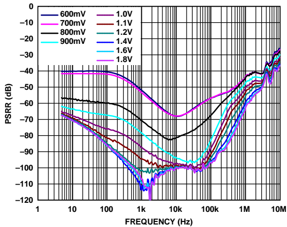
Figure 24. Power Supply Rejection Ratio (PSRR) vs. Frequency for Various Headroom Voltages, ADM7151-04, V_{OUT} = 5 V , 400 mA Load
