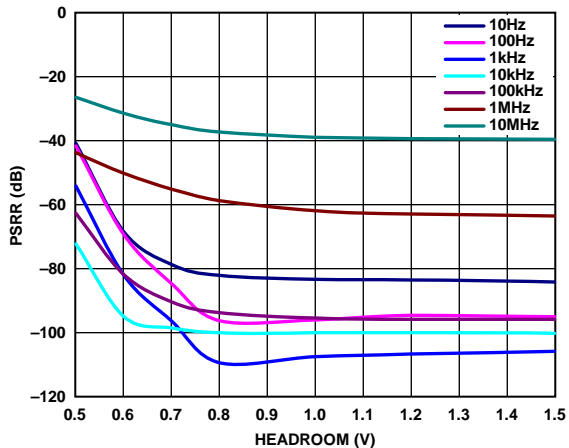
Figure 25. Power Supply Rejection Ratio (PSRR) vs. Headroom Voltage, ADM7151-02, V_{OUT} = 4 V , 100 mA Load
