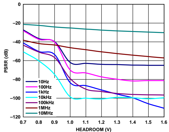
Figure 27. Power Supply Rejection Ratio (PSRR) vs. Headroom Voltage, ADM7151-02, V_{OUT} = 4 V , 800 mA Load
