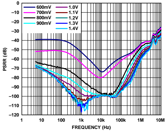
Figure 23. Power Supply Rejection Ratio (PSRR) vs. Frequency for Various Headroom Voltages, ADM7151-02, V_{OUT} = 4 V , 400 mA Load
