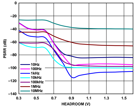
Figure 28. Power Supply Rejection Ratio (PSRR) vs. Headroom Voltage, ADM7151-04, V_{OUT} = 5 V , 100 mA Load
