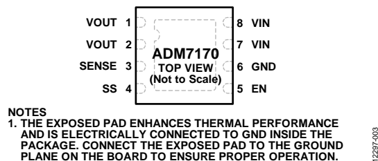
Figure 3. Pin Configuration
