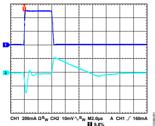
Figure 51. Load Transient Response, I_{LOAD} = 10mA to 500 mA, Adjustable Version, V_{OUT} = 1.2V , V_{IN} = 2.5V , CH1 = I_{LOAD} , CH2 = V_{OUT}
