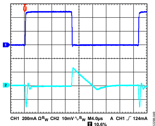
Figure 49. Load Transient Response, I_{LOAD} = 10mA to 500 mA, V_{OUT} = 5V , V_{IN} = 5.5V , CH1 = I_{LOAD} , CH2 = V_{OUT}
