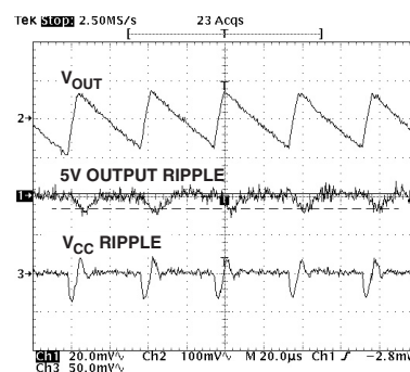
TPC 9. Output Ripple on LDO (5V Output)
