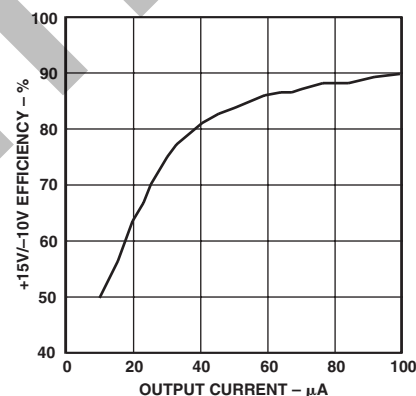
TPC 6. +15V/-10V Efficiency vs. Output Current in Scanning Mode, V_{CC} = 3\text{ V}
