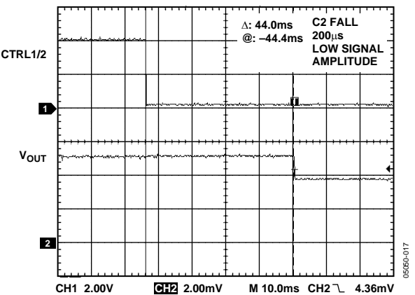
Figure 16. TPC Delay
