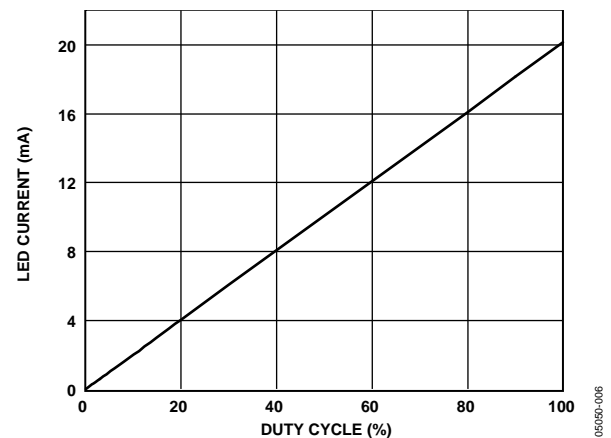
Figure 5. I_{LED} (mA) vs. PWM Dimming (Varying Duty Cycle), Four LEDs Enabled, Frequency = 1 kHz
