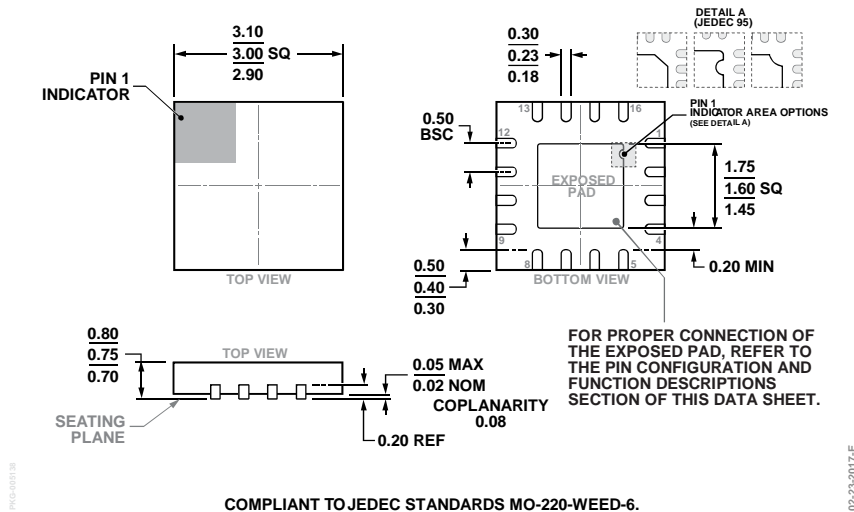
Figure 31. 16-Lead Lead Frame Chip Scale Package [LFCSP] 3 mm × 3 mm Body and 0.75 mm Package Height (CP-16-22)
