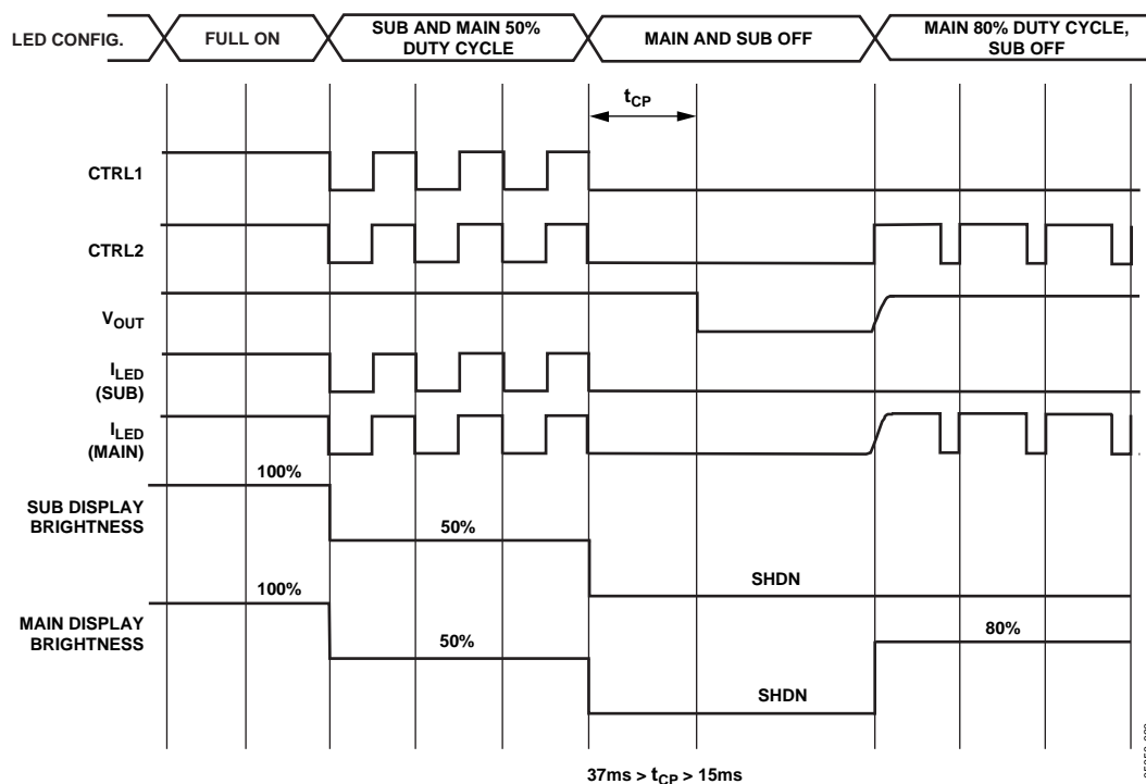
Figure 20. Application Timing
