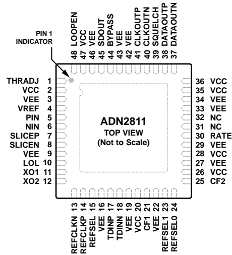
Figure 2. Pin Configuration
