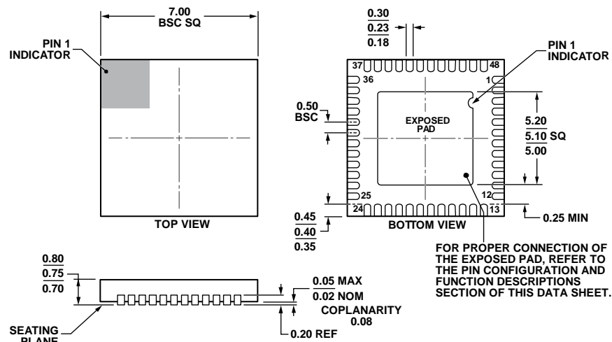
Figure 26. 48-Lead Lead Frame Chip Scale Package [LFCSP] 7 mm × 7 mm Body and 0.75 mm Package Height (CP-48-4)
