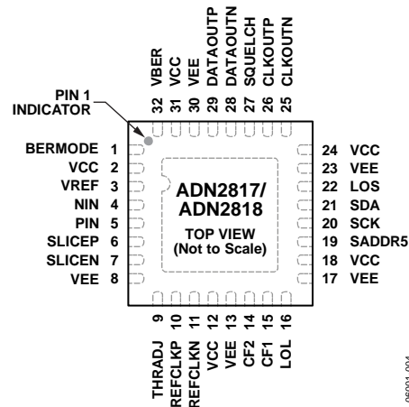
Figure 5. Pin Configuration
