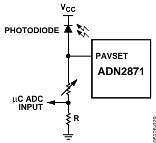
Figure 34. Single Measurement of I_{IMPD} Across a Sense Resistor in Resistor Setpoint I_{IMPD} Monitoring
