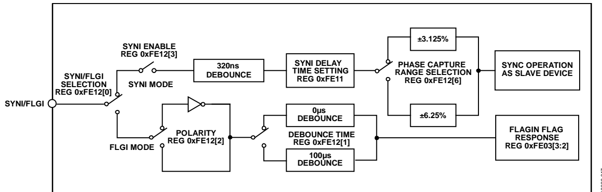
Figure 16. Synchronization Configuration
