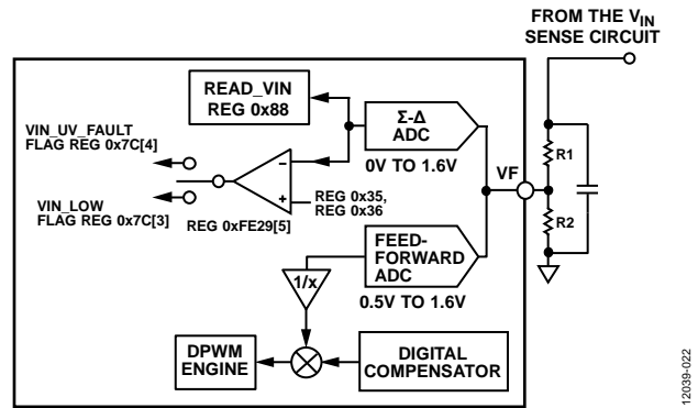
Figure 20. Closed-Loop Input Voltage Feedforward Configuration
