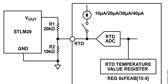
Figure 30. Temperature Sensing by an Analog Temperature Sensor
