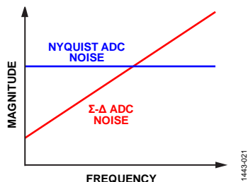
Figure 21. ADC Noise Performance
