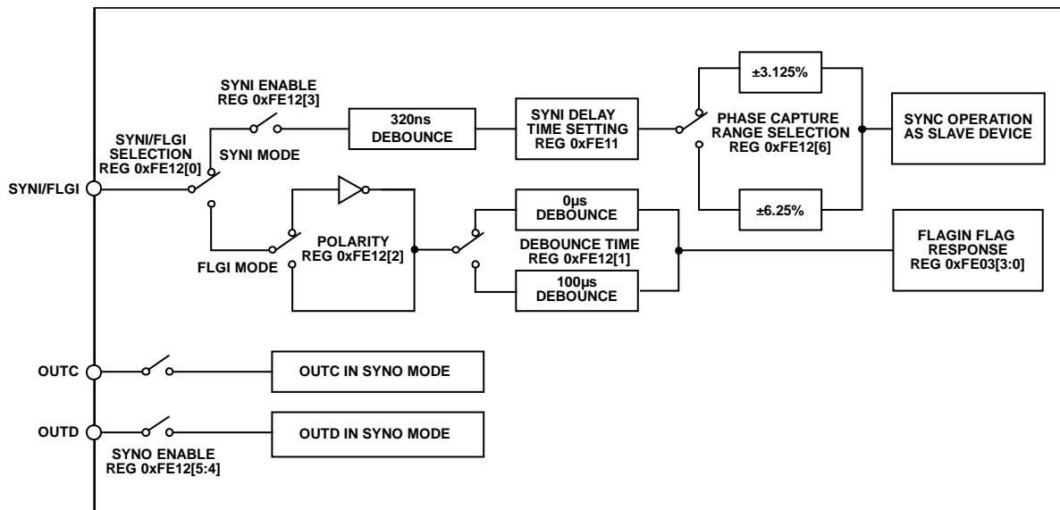
Figure 18. Synchronization Configuration
