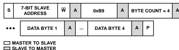
Figure 60. Write Four Bytes to Page 9
