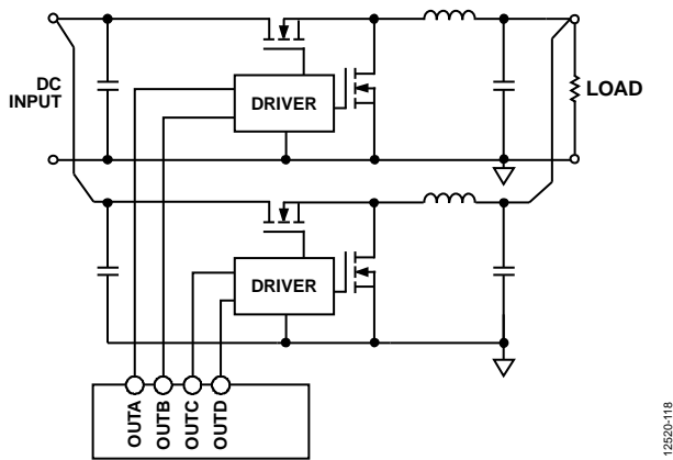
Figure 15. Dual-Phase Interleaved Buck Converter Controlled by the ADP1052
