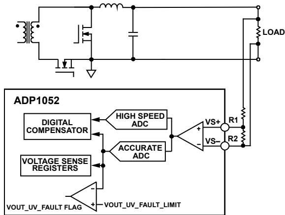
Figure 20. Voltage Sense Configuration
