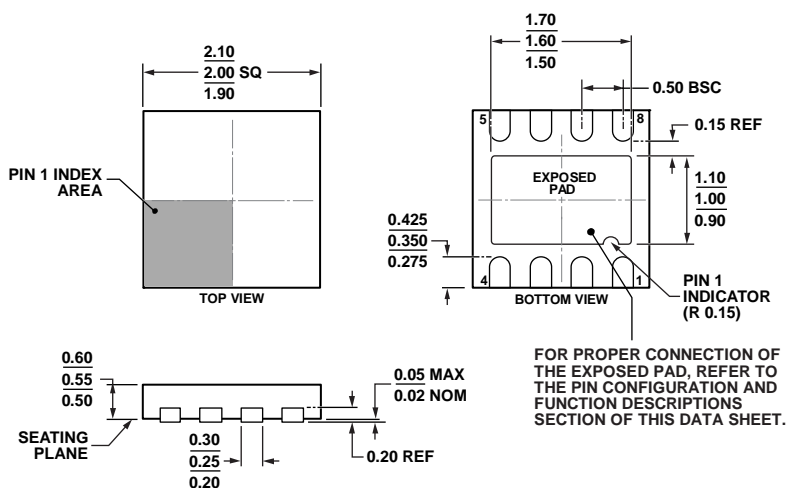
Figure 46. 8-Lead Lead Frame Chip Scale Package [LF CSP_UD] 2 mm × 2 mm Body, Ultra Thin, Dual Lead (CP-8-10)
