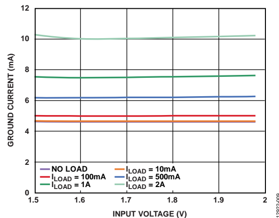
Figure 9. Ground Current vs. Input Voltage
