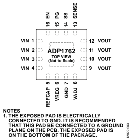
Figure 3. Pin Configuration
