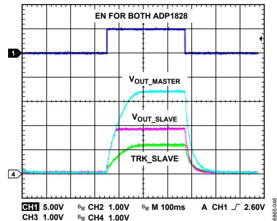
Figure 45. Coincident Tracking of Figure 43
