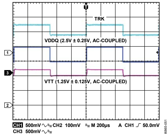
Figure 50. DDR Termination; Output Waveforms of Figure 49
