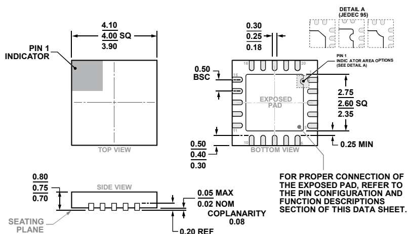
Figure 59. 20-Lead Lead Frame Chip Scale Package (LFCSP) 4 mm × 4 mm Body and 0.75 mm Package Height (CP-20-8)
