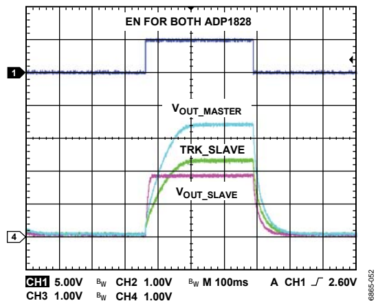
Figure 51. Ratiometric Tracking of Figure 47 with R_{TRKT} = 5 \text{ k}\Omega
