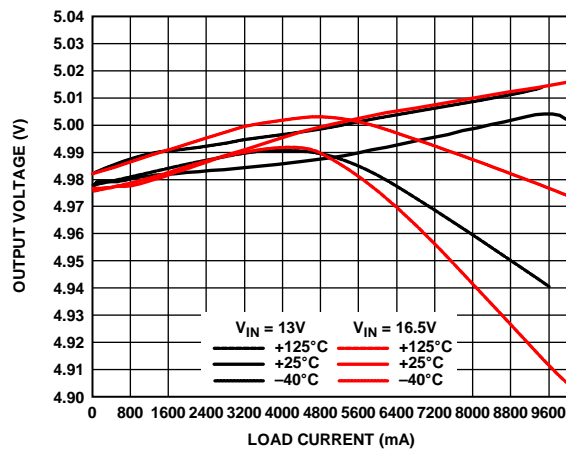
Figure 21. Output Voltage Accuracy—1.0 MHz, V_{OUT} = 5\text{ V}
