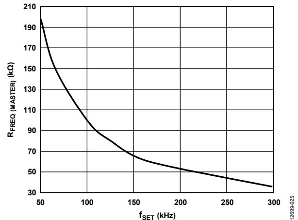
Figure 28. R_{FREQ(MASTER)} vs. Switching Frequency ( f_{SET} )
