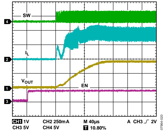
Figure 19. Startup, V_{OUT} = 1.8\text{ V} , 400 mA
