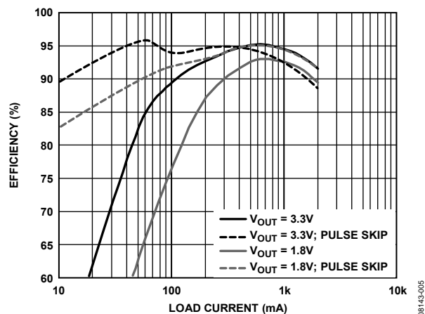
Figure 5. Channel 2 Efficiency vs. Load, V_{IN} = 5V and f_{SW} = 600\text{ kHz} ; V_{OUT} = 3.3V , Inductor TOKO FDV0620-4R7M, 4.7\mu H , 53\text{ m}\Omega ; V_{OUT} = 1.8V , Inductor TOKO FDV0620-2R2M, 2.2\mu H , 30\text{ m}\Omega
