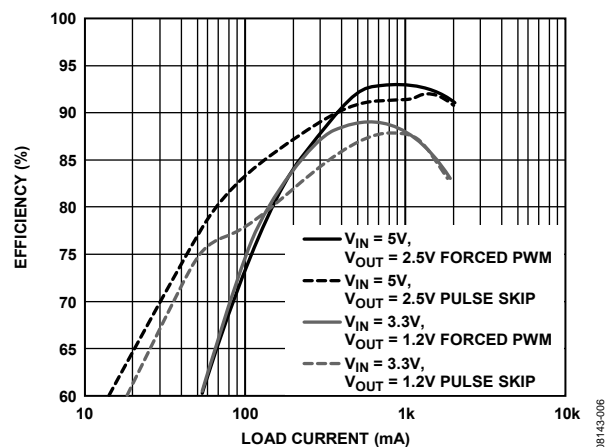
Figure 6. Efficiency vs. Load at f_{SW} = 1.2\text{ MHz} ; Inductor TOKO FDV0620-1R0M, 1.0\mu H , 14\text{ m}\Omega
