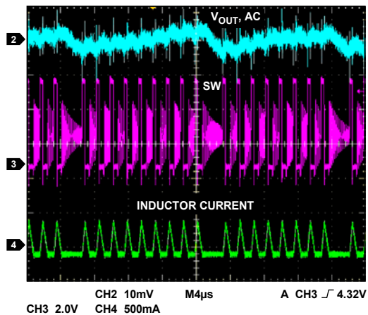
Figure 49. Pulse Skip Mode, 110 mA Load
