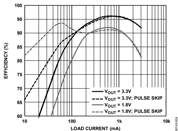
Figure 4. Channel 1 Efficiency vs. Load, V_{IN} = 5V and f_{SW} = 300\text{ kHz} ; V_{OUT} = 3.3V , Inductor Cooper Bussmann DR1050-8R2-R, 8.2\mu H , 15\text{ m}\Omega ; V_{OUT} = 1.8V , Inductor TOKO FDV0620-4R7M, 4.7\mu H , 53\text{ m}\Omega
