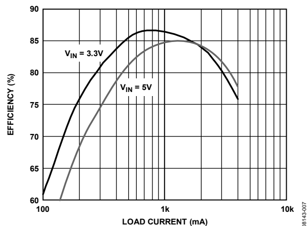
Figure 7. Efficiency Combined Dual-Phase Output, V_{OUT} = 0.8V and f_{SW} = 1.2\text{ MHz} ; Inductor TOKO FDV0620-1R0M, 1.0\mu H , 14\text{ m}\Omega
