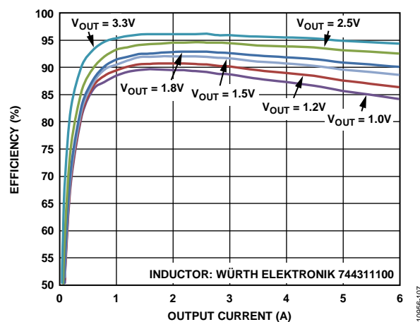
Figure 8. Efficiency ( f_{SW} = 600\text{ kHz} , V_{PVIN} = 5\text{ V} ) vs. Output Current
