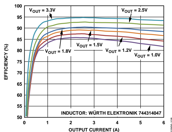
Figure 9. Efficiency ( f_{SW} = 1.2\text{ MHz} , V_{PVIN} = 5\text{ V} ) vs. Output Current
