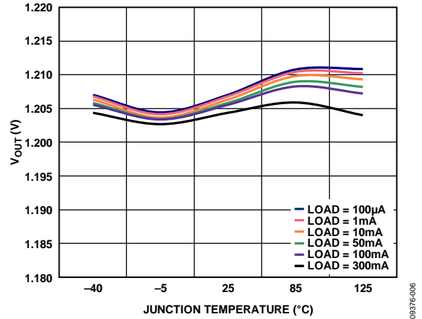
Figure 26. Output Voltage vs. Junction Temperature, V_{OUTx} = 1.2\text{ V} , ADP223/ADP225
