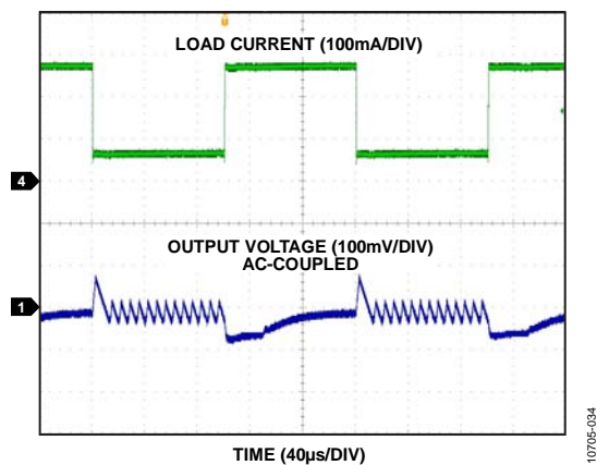
Figure 21. Load Transient Response, V_{OUT} = 3.3 V, Auto Mode, 50 mA to 250 mA
