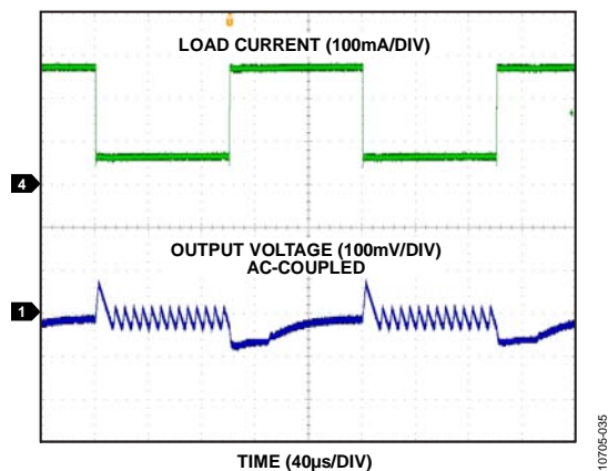
Figure 22. Load Transient Response, V_{OUT} = 3.3 V, Auto Mode, 200 mA to 600 mA
