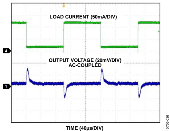
Figure 23. Load Transient Response, V_{OUT} = 1.8 V, PWM Mode, 10 mA to 110 mA
