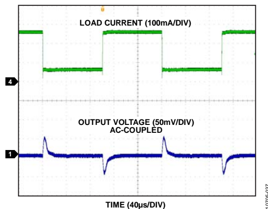
Figure 24. Load Transient Response, V_{OUT} = 1.8 V, PWM Mode, 50 mA to 250 mA
