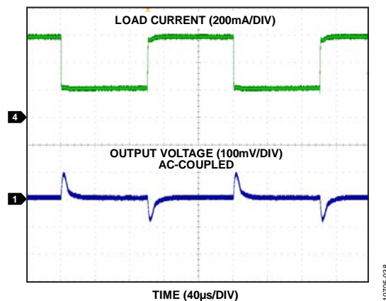
Figure 25. Load Transient Response, V_{OUT} = 1.8 V, PWM Mode, 200 mA to 600 mA
