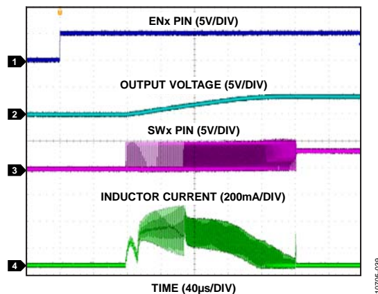
Figure 26. Startup, V_{OUT} = 3.3 V, No Load
