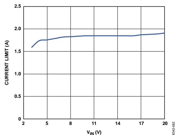
Figure 20. Current-Limit Threshold vs. V_{IN} , V_{BST} - V_{SW} = 5.0\text{ V}
