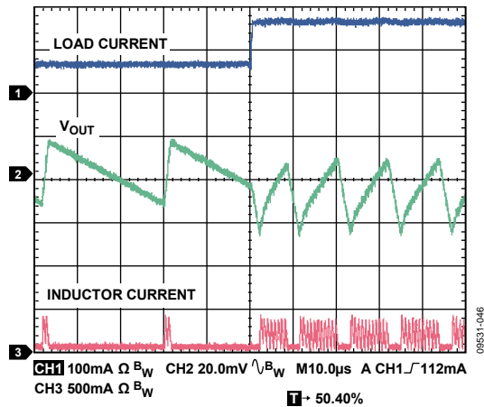
Figure 46. Load Transient, V_{OUT} = 1.2 V, 10 mA to 110 mA, Load Current Rise Time = 200 ns, V_{IN} = 5 V
