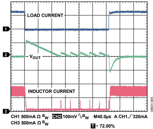
Figure 45. Load Transient, V_{OUT} = 1.2 V, 10 mA to 800 mA, Load Current Rise Time = 200 ns, V_{IN} = 5 V
