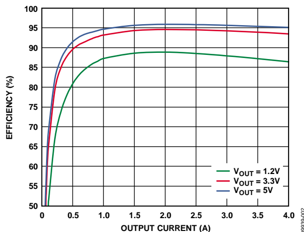
Figure 2. Efficiency vs. Output Current, V_{IN} = 12\text{ V} , f_{SW} = 250\text{ kHz}
