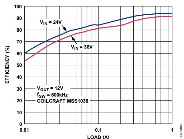
Figure 15. Efficiency vs. Load Current, V_{OUT} = 12\text{ V} , f_{SW} = 600\text{ kHz}
