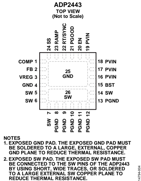
Figure 4. Pin Configuration
