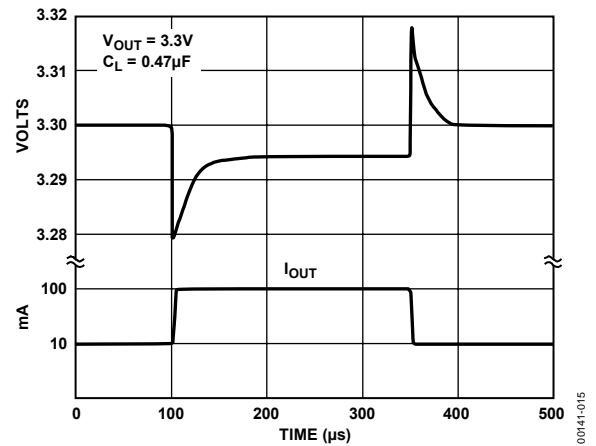
Figure 15. Load Transient
