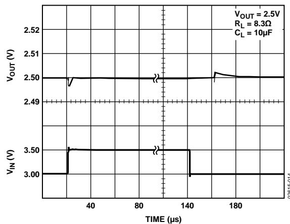
Figure 14. Line Transient Response, C_L = 10 \mu F
