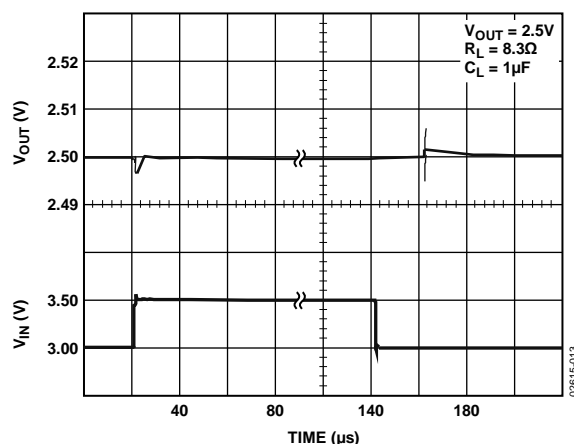
Figure 13. Line Transient Response, C_L = 1 \mu F
