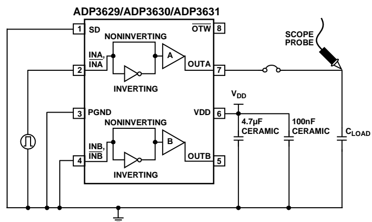
Figure 20. Test Circuit
