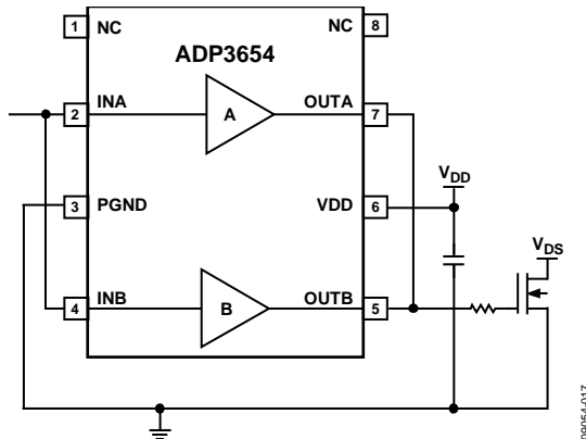
Figure 17. Parallel Operation
