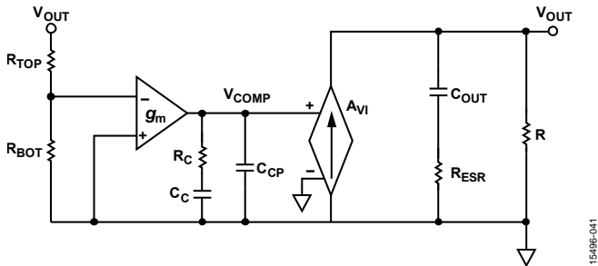
Figure 40. Simplified Peak Current-Mode Control Small Signal Circuit
