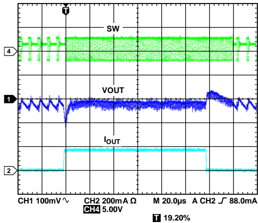
Figure 28. BUCK2 Response to Load Transient, I_{OUT2} = 20 \text{ mA} to 180 \text{ mA} , V_{OUT2} = 1.8 \text{ V} , Auto Mode
