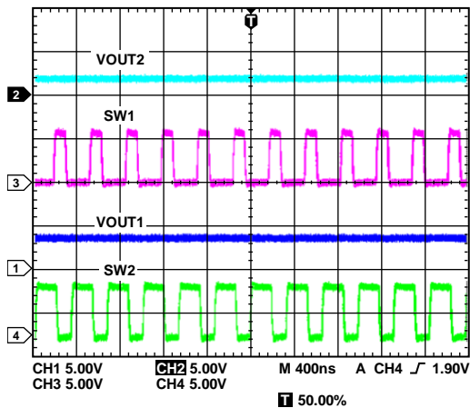
Figure 29. VOUT and SW Waveforms for BUCK1 and BUCK2 in PWM Mode Showing Out-of-Phase Operation
