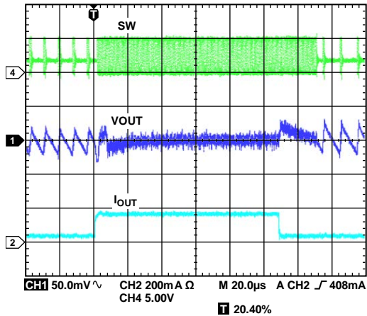
Figure 27. BUCK1 Response to Load Transient, I_{OUT1} = 20 \text{ mA} to 180 \text{ mA} , V_{OUT1} = 3.3 \text{ V} , Auto Mode
