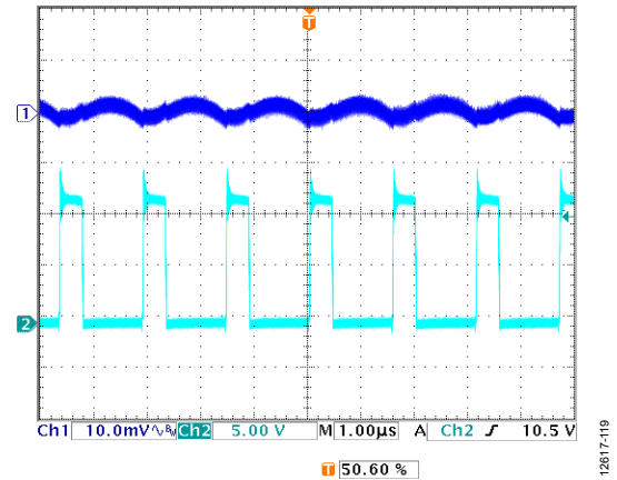
Figure 19. Steady State Waveform at Heavy Load, V_{IN} = 12V , V_{OUT} = 3.3V , I_{OUT} = 3A , f_{SW} = 600kHz , L = 4.7\mu H , C_{OUT} = 47\mu F \times 2 , FPWM Mode, Channel 1 = V_{OUTx} , Channel 2 = SWx
