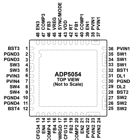
Figure 3. Pin Configuration
