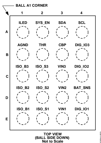
Figure 3. Pin Configuration
