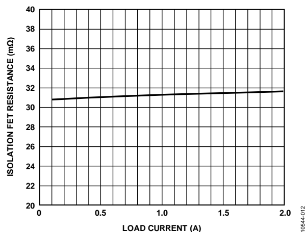
Figure 12. Ideal Diode R_{ON} vs. Load Current, V_{ISO\_B} = 3.6 V
